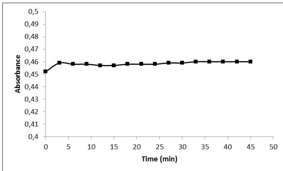
Fig. 2. Effect of time on the color stability of the reduced phosphomolybdate complex solution from the solution of 50 mL of 0.8 mg P/L phosphate working solution and 8 mL of mixed solution
