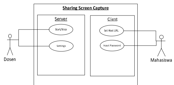
Gambar 2. Use Case Diagram Aplikasi Sharing Screen Capture
