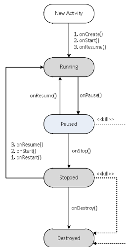
Gambar 3. Lifecycle Activity Aplikasi Sharing Screen Capture
