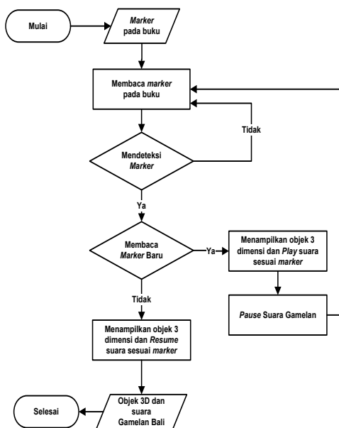
Gambar 1. Flowchart Aplikasi Augmented Reality Book Pura Batur
