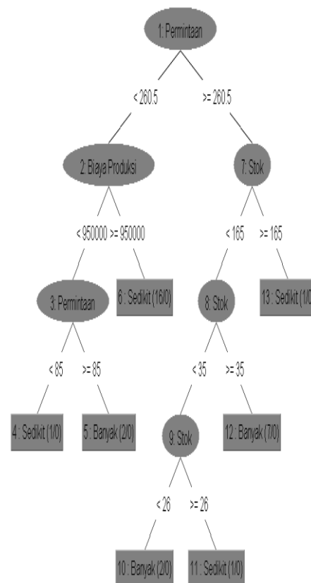
Gambar 3. Pohon Keputusan Random Tree
