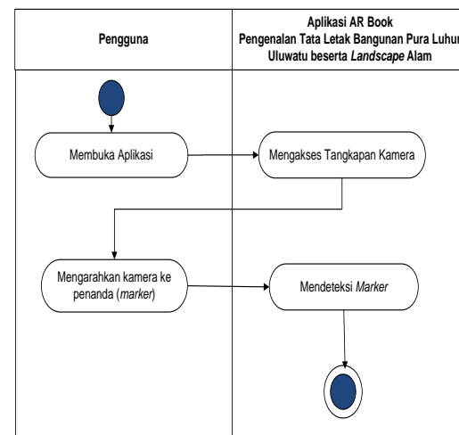
Gambar 4a. Activity Diagram Melacak Marker
