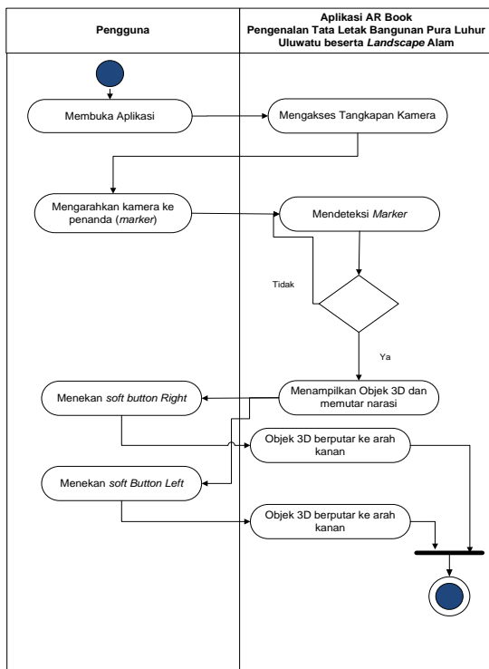
Gambar4c. Activity Diagram Merotasikan Objek 3D
