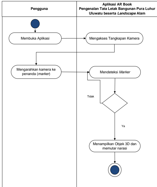
Gambar4b. Activity Diagram Menampilkan Objek 3D
