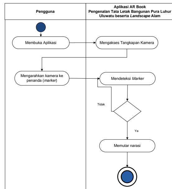
Gambar4e. Activity diagram Memutar Narasi
