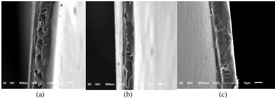
Gambar 6. Citra/image SEM membran PEC kitosan-pektin a: (70:30), b (80:20), c (90:10)
